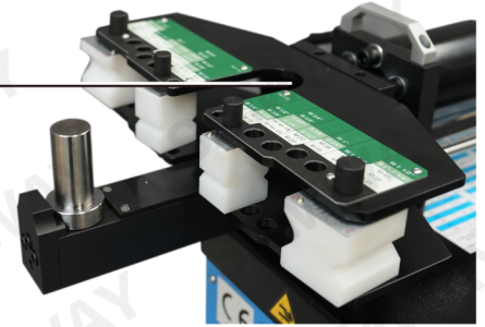
Bending Modular
